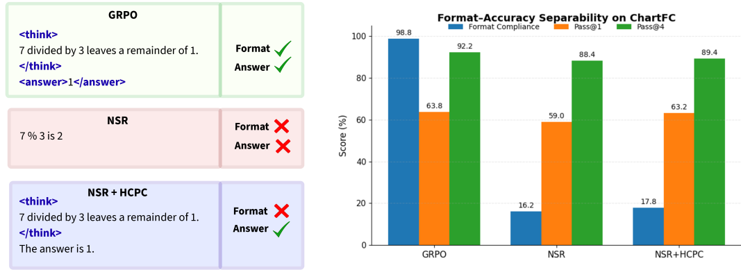
Figure 1: Format and answer accuracy are separable channels in chart RLVR. Left: a stylized rollout under each training regime. GRPO emits the required structural tags and the correct answer; NSR drops both; NSR+HCPC recovers the answer while the structured tags remain collapsed. Right: ChartFC (OOD) metrics for the same three regimes. Adding HCPC on top of NSR restores Pass@1 and Pass@4 to near GRPO levels, but format compliance barely moves from NSR’s collapsed value (16.2% to 17.8%). Accuracy returns; format does not. The dissociation is direct evidence that these two behaviors respond independently to training interventions.
